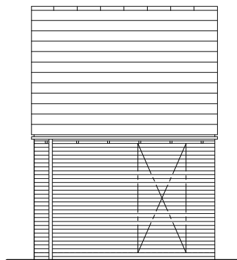
REAR ELEVATION
